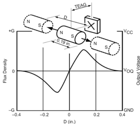
Figure 3. Slide-by sensor actuation. TEAG is the total effective air gap.
