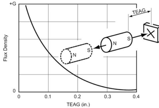
Figure 2. Head-on Hall sensor actuation. TEAG is the total effective air gap.
