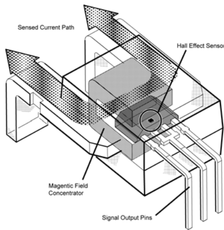
Figure 7. Current sensor Hall device for high current (> 200 A) applications.
