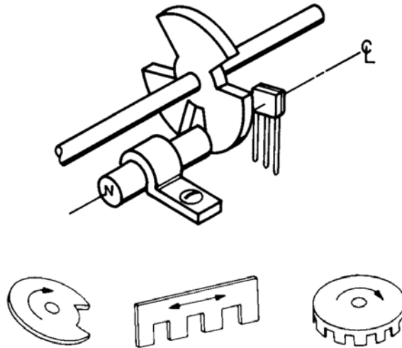
Figure 4. Vane interrupter switching Hall sensor actuation.
