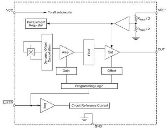
Figure 12: Block diagram of the 3V, A139x micro-power linear with sleep pin input.
