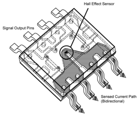
Figure 6. Current sensor Hall device in SOIC-8 package.
