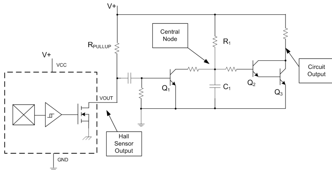
Figure 11: Broken belt detection circuit using simple Hall switch.
