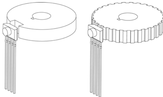
Figure 5. Gear tooth Hall sensor actuation.
